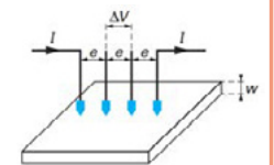
Conductivity measurement with the four-probe system
